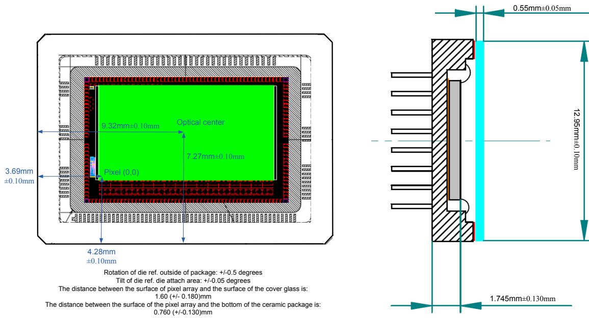
Figure 36: Assembly drawing of CMV2000.
