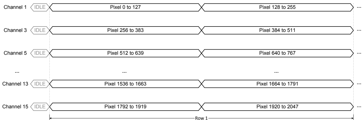
Figure 21: Pixel remapping for 8 output channels
