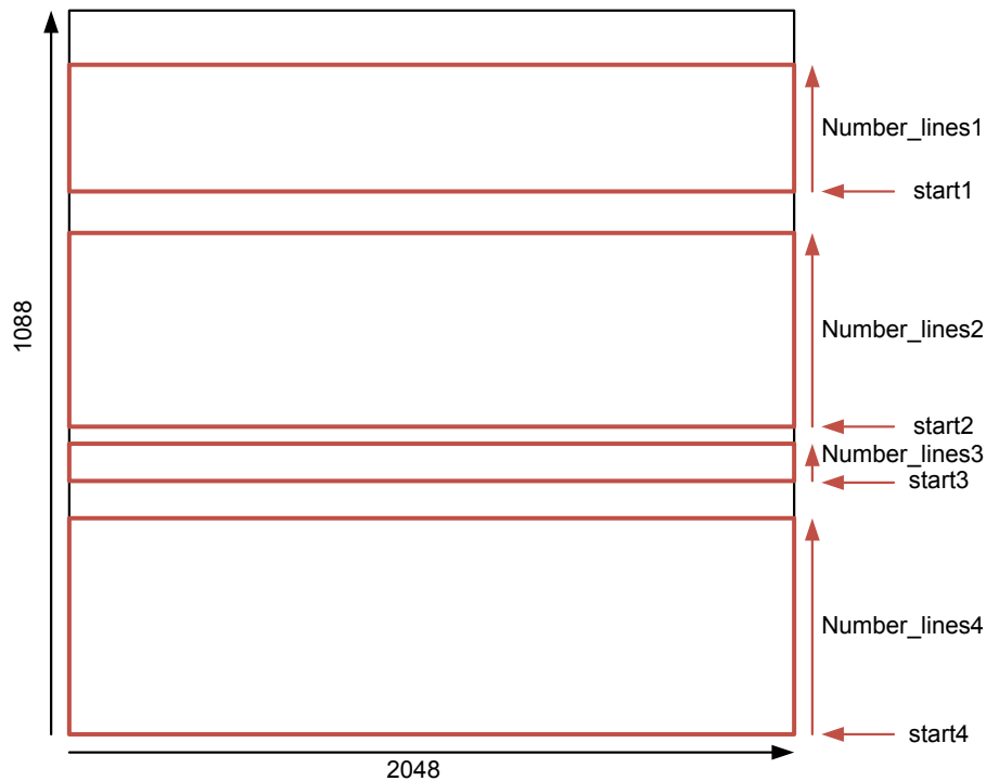
Figure 32: Example of 4 multiple frames read-out
