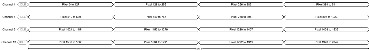
Figure 22: Pixel remapping for 4 output channels
