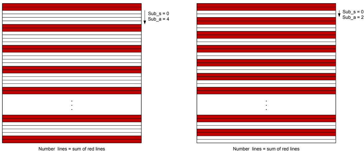
Figure 34: Subsampling examples in advanced mode (skip 4x and skip2x)
