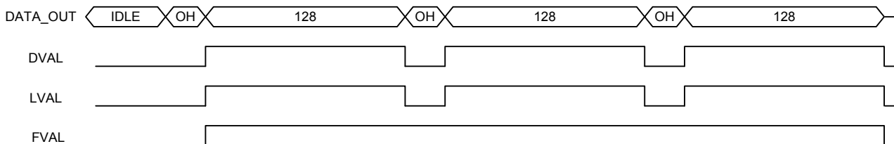
Figure 24: DVAL, LVAL and FVAL timing in 16 output mode
