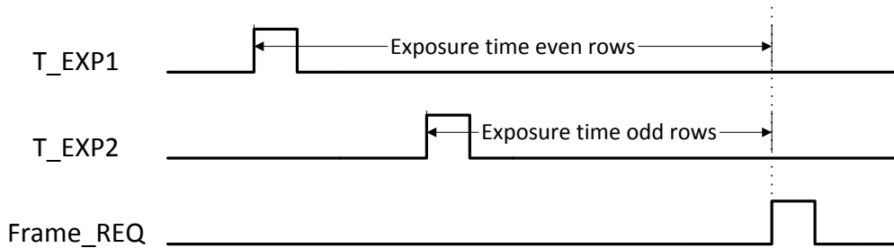
Figure 27: Interleaved read-out in external exposure mode
