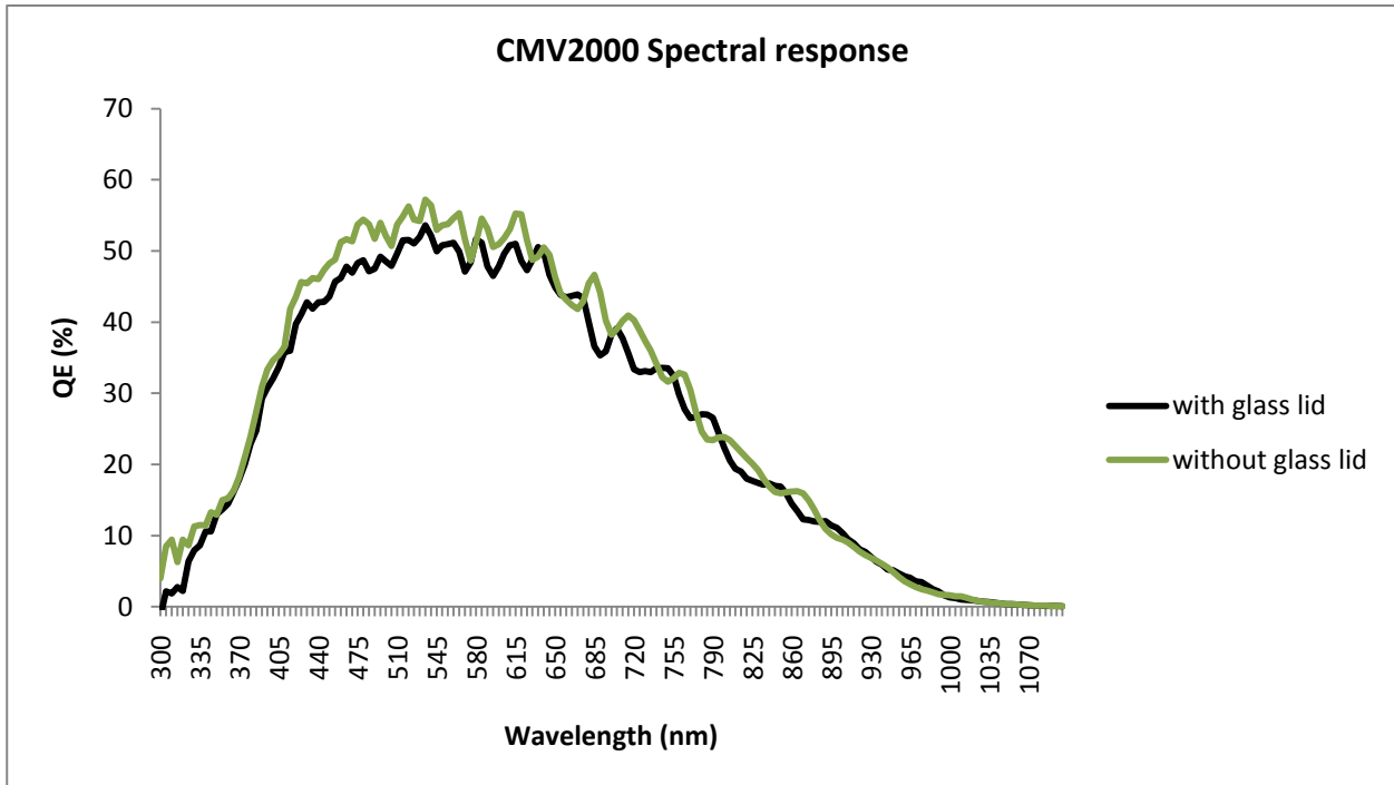
Figure 39: Typical spectral response of the CMV2000
