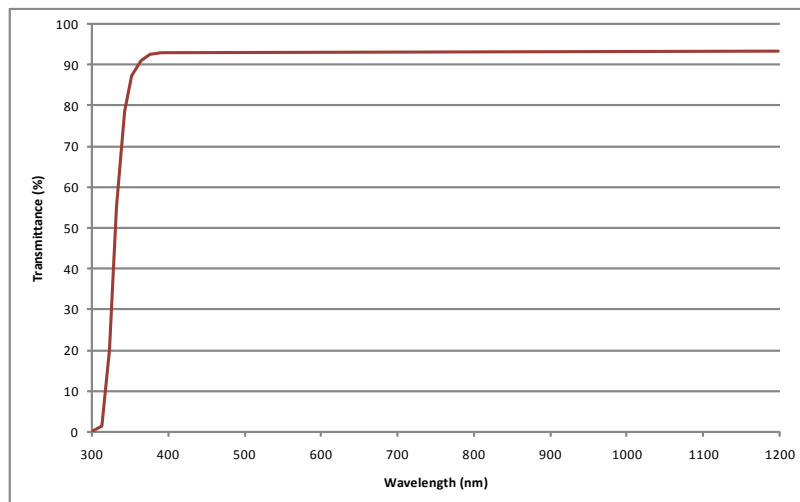
Figure 37: Transmittance curve of D263 cover glass
