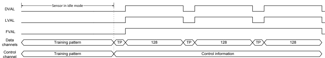
Figure 26: Training pattern location in the data and control channels.
