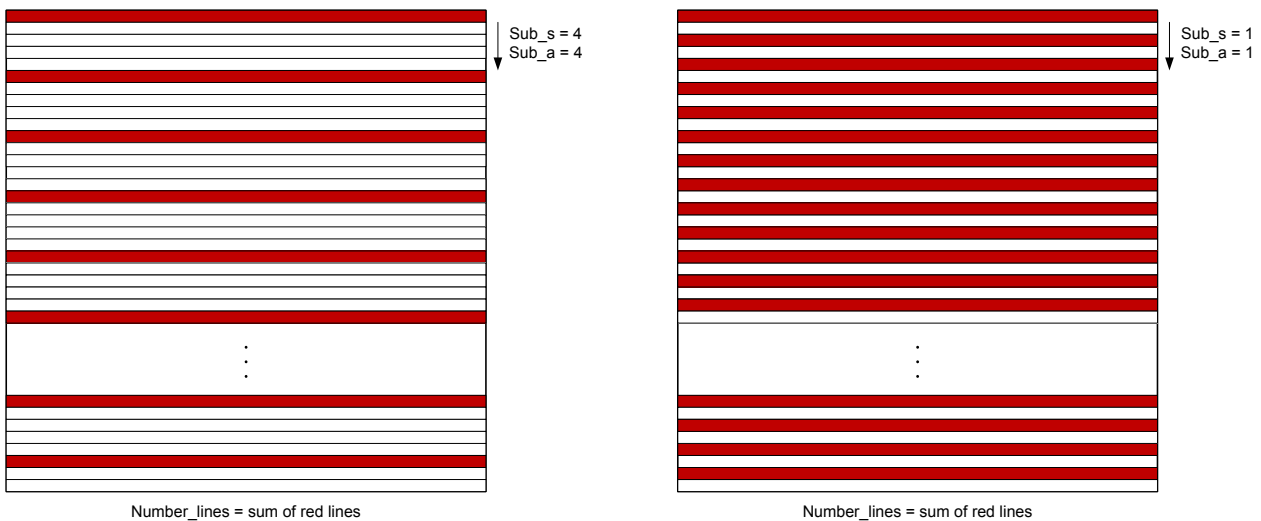
Figure 33: Subsampling examples (skip 4x and skip 1x)
