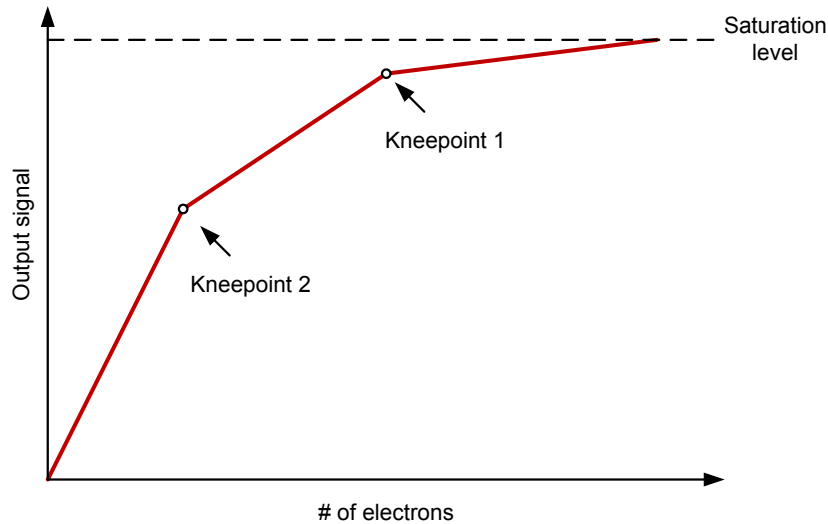
Figure 29: Piecewise linear response
