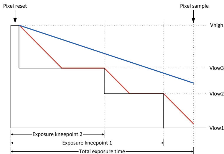
Figure 28: Piecewise linear response details
