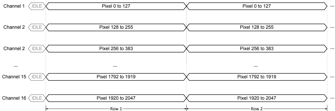
Figure 20: Pixel remapping for 16 output channels
