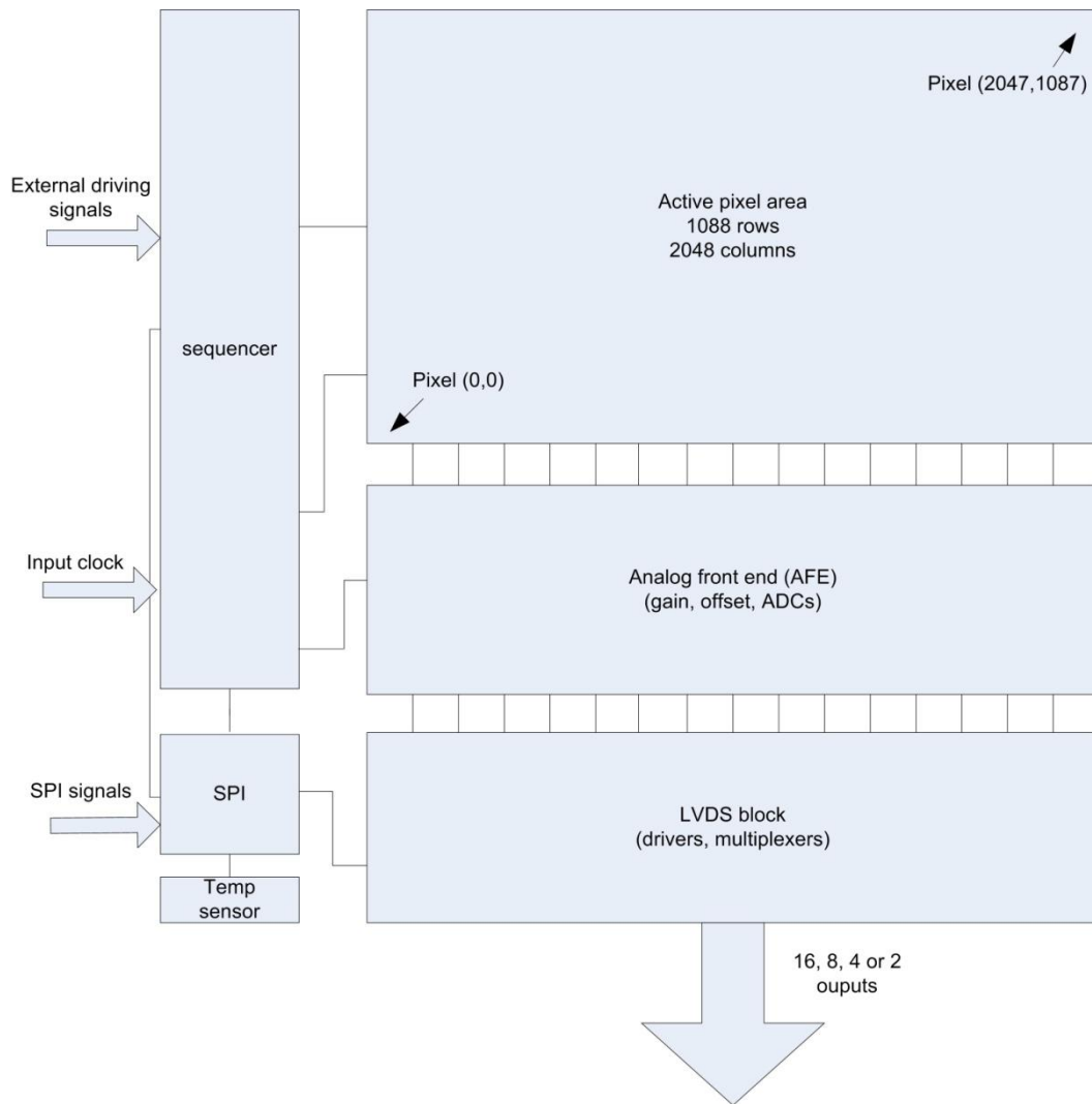
Figure 2: Sensor block diagram
