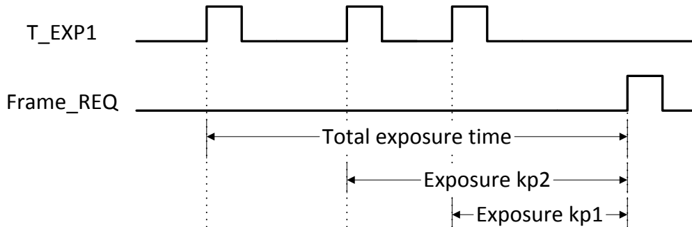
Figure 30: Piecewise linear response with external exposure time mode
