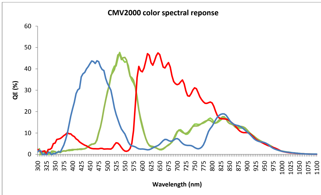
Figure 38: Typical spectral response of CMV2000 with RGB color filters and D263 cover glass
